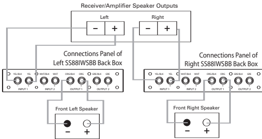
Connection Method #1, Using Two SS881WS Loudspeakers With Back Boxes (Use Shorting Straps)
